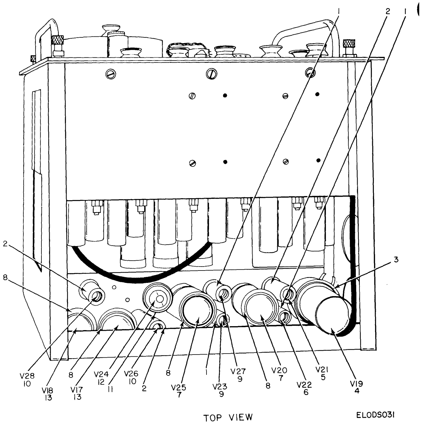
Figure 29. Test Set, Radar TS-743/UPM, Panel-Chassis, Top View.
