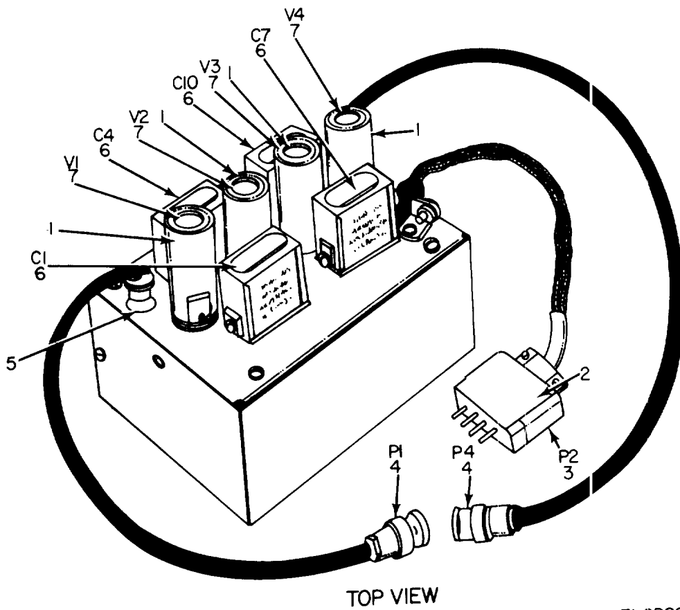
Figure 38. Crystal Amplifier Assembly (Sheet 1 of 3).
