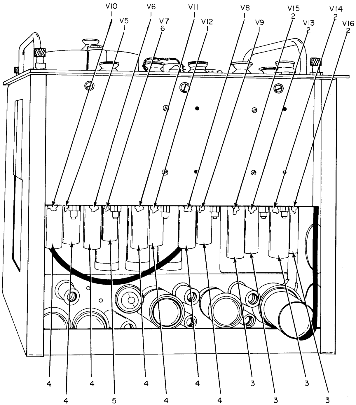
Figure 34. Modulator Assembly, Top View.
