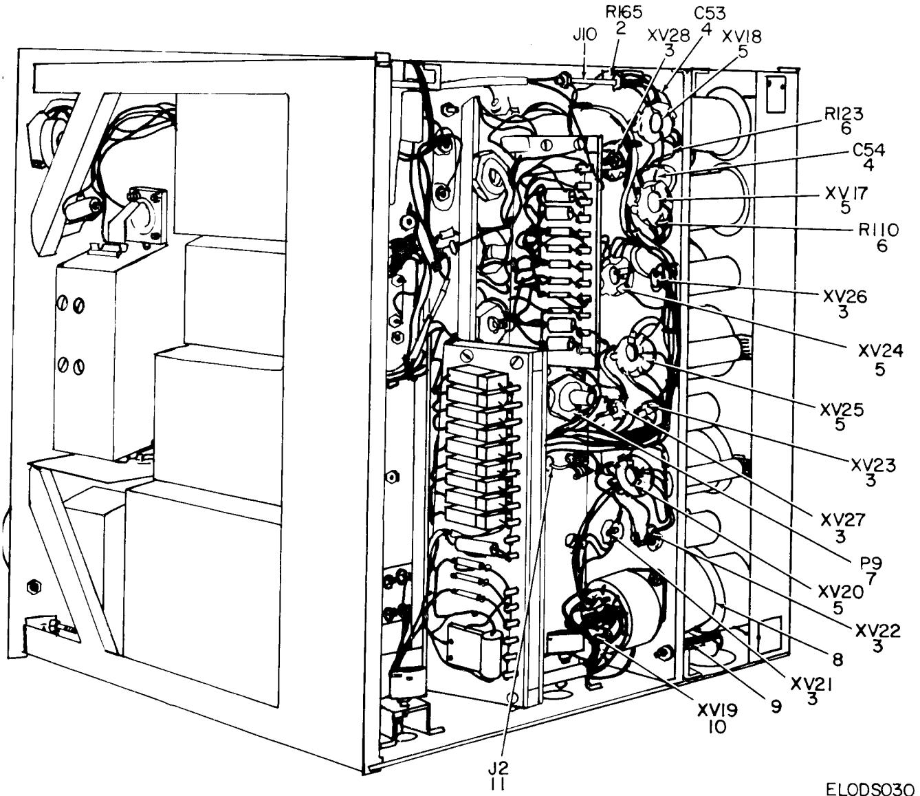
Figure 28. Test Set, Radar TS-743/UPM, Rear of Panel-Chassis, Right Oblique View.
