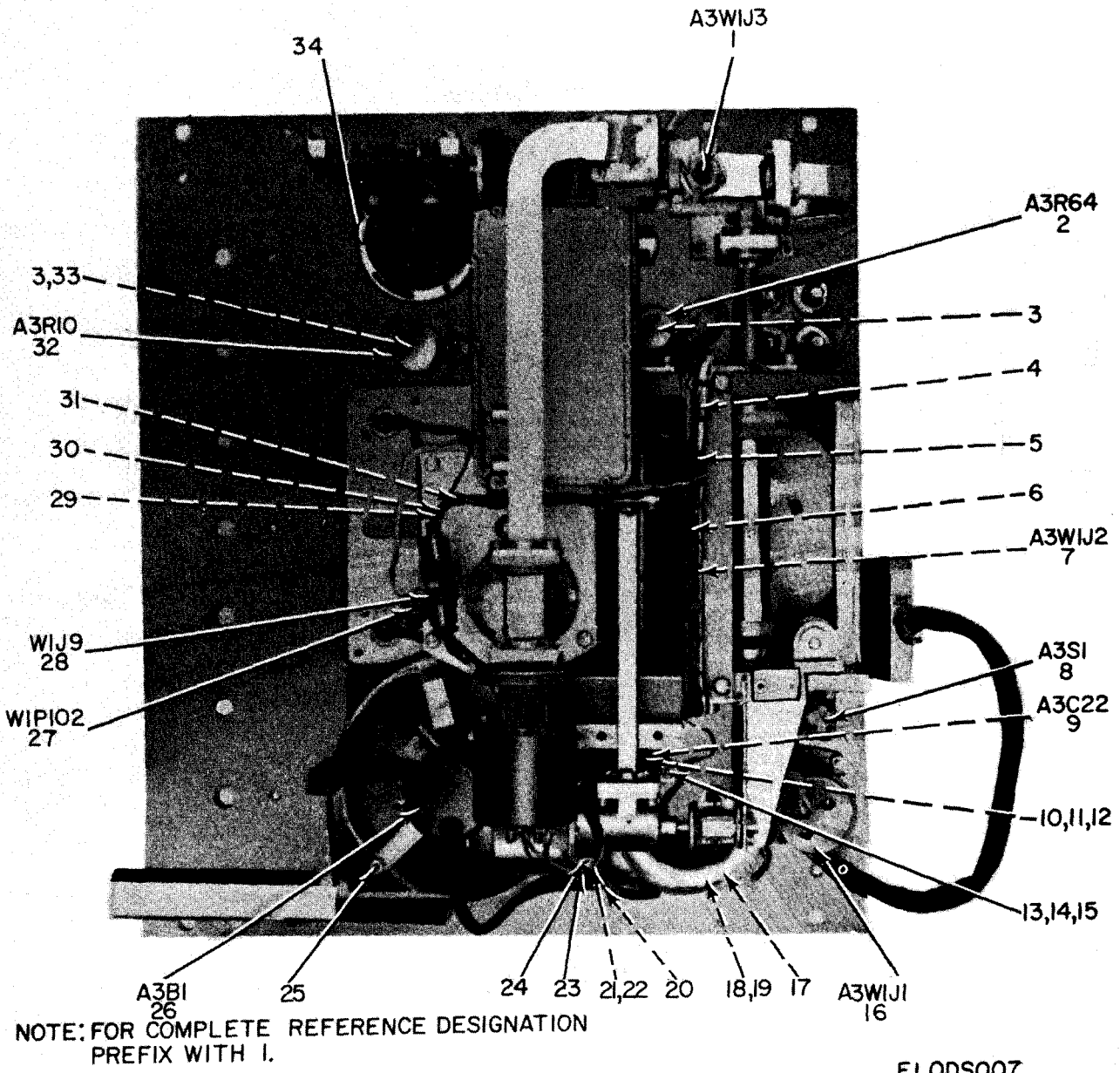
Figure 6. Test Set, Radar TS-743A/UPM, Panel Assembly, Rear View.
