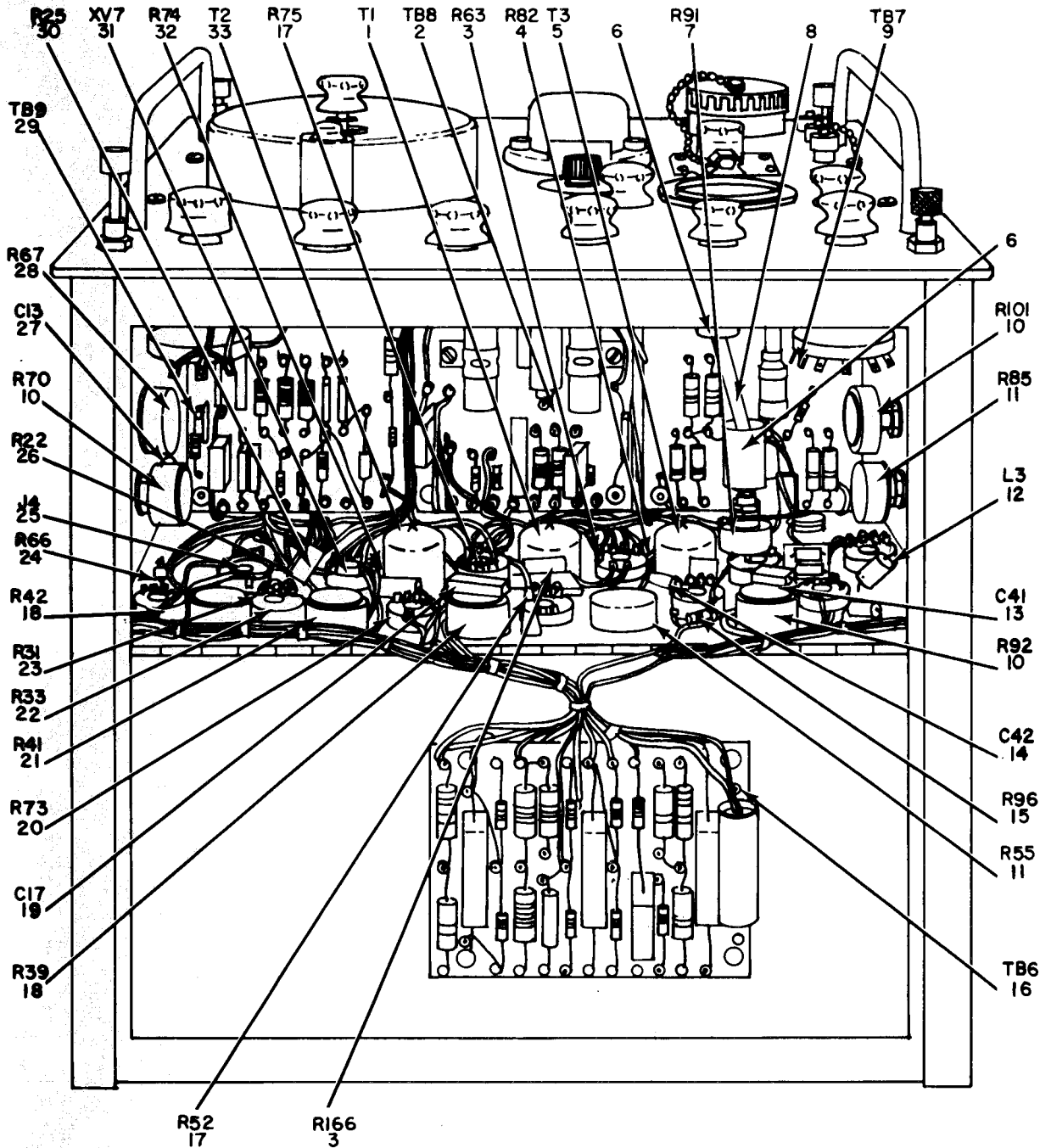
COMPONENT LOCATION
