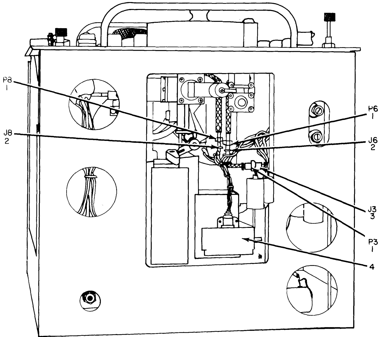
Figure 35. Modulator Assembly, Right Side View.
