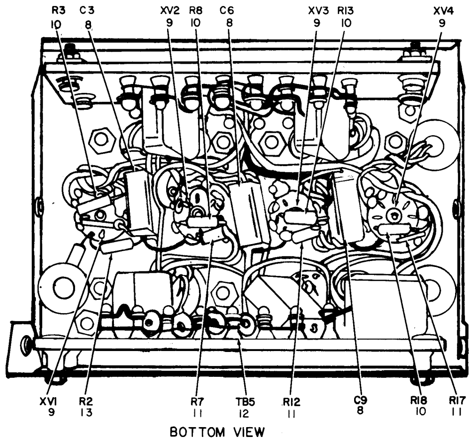
Figure 38. Crystal Amplifier Assembly (Sheet 2 of 3).
